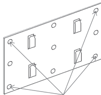
Use screws to fasten bracket to building structure
